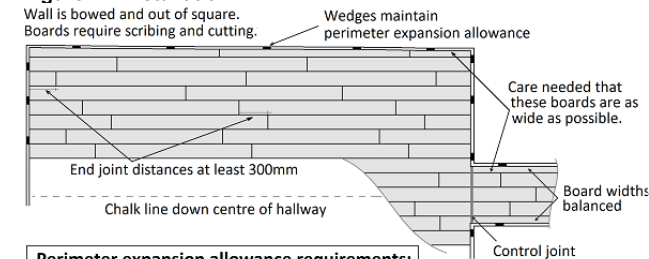
Figure 2 – Installation
