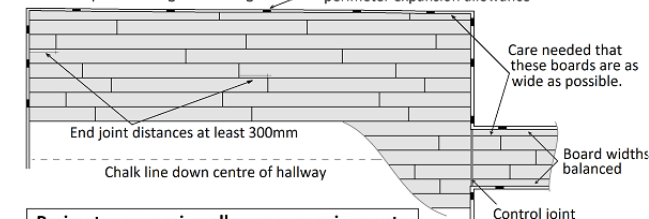
Figure 2 – Installation
