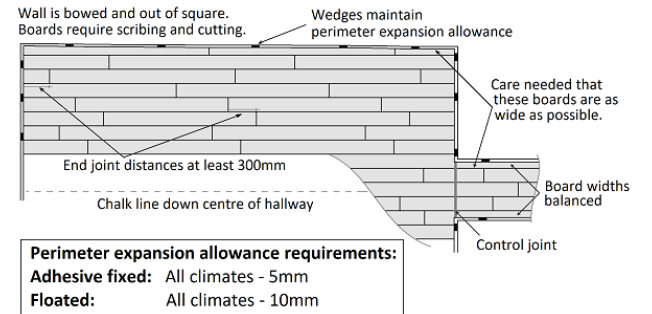
Figure 3 – Scribing
