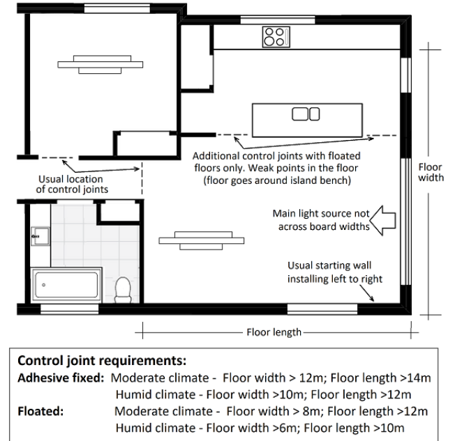
Figure 2 – Installation
