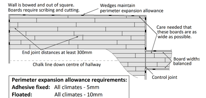
Figure 3 – Scribing
