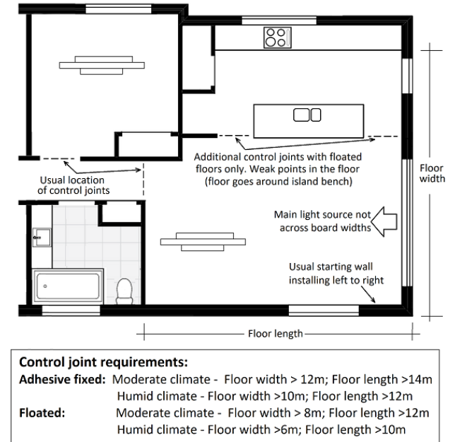
Figure 2 – Installation
